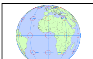
Vertical Near Side Perspective 外射図法
